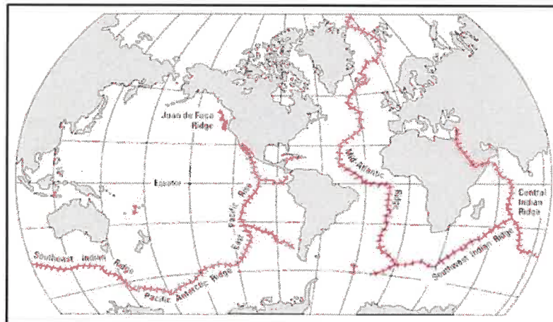
Fig. 4. Sistemul de rifturi al Terrei (Sursa: https://oceanclass.blogspot.com/2011/08/4-tectonica-placilor-relieful.html )
